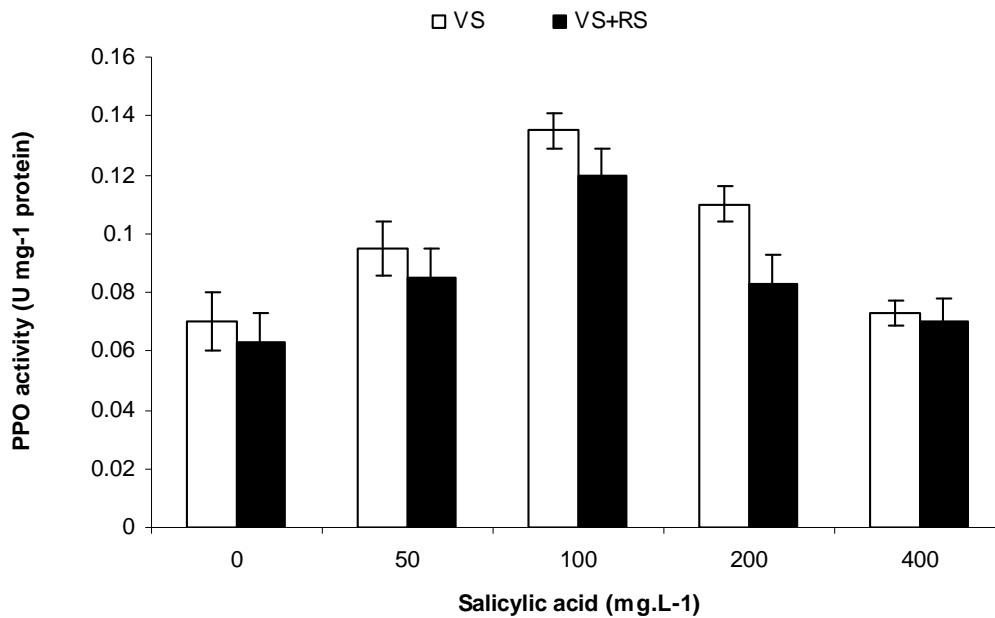
Fig. 2 - Variations of polyphenol oxidase (PPO) activity in Satureja khuzistanica under different salicylic acid concentration and spraying time (VS: Vegetative stage, RS: Reproductive stage). The error bars represent the standard deviation ( \pm SD) for replicates (n=3)
