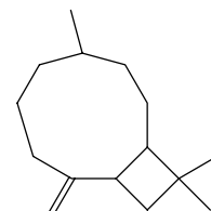
\beta -Caryophyllene
