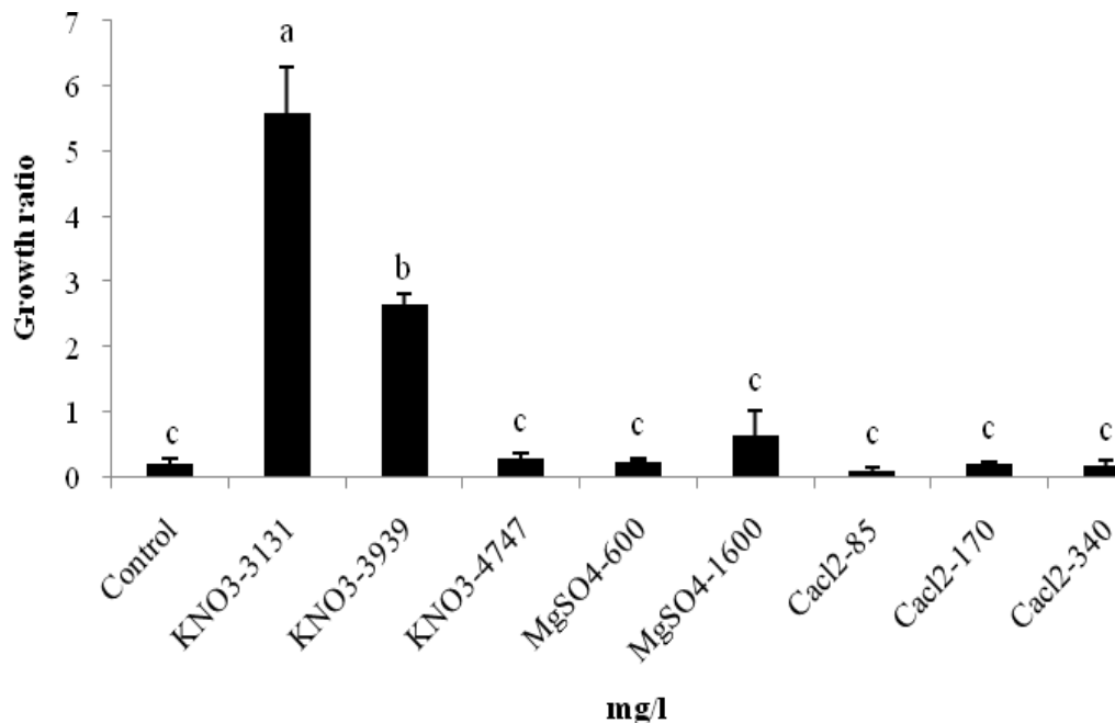
Figure 2- Effects of MS macro-elements concentrations on hairy roots growth in Echinacea purpurea
