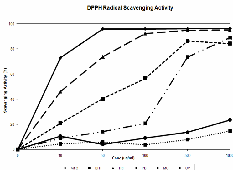
Fig. 1- DPPH radical scavenging activity of TRF, PB, MC and CV. 20 \mu\text{g/ml} of DPPH solution was added to TRF, PB, MC and CV at a ratio of 1:1 before 30 minutes incubation at room temperature. Vitamin C and BHT represent DPPH standards, while TRF acts as positive control. TRF exhibit a stronger scavenging activity compared to BHT, followed by PB, MC and CV extracts. Data is presented as means \pm SD, n=9
