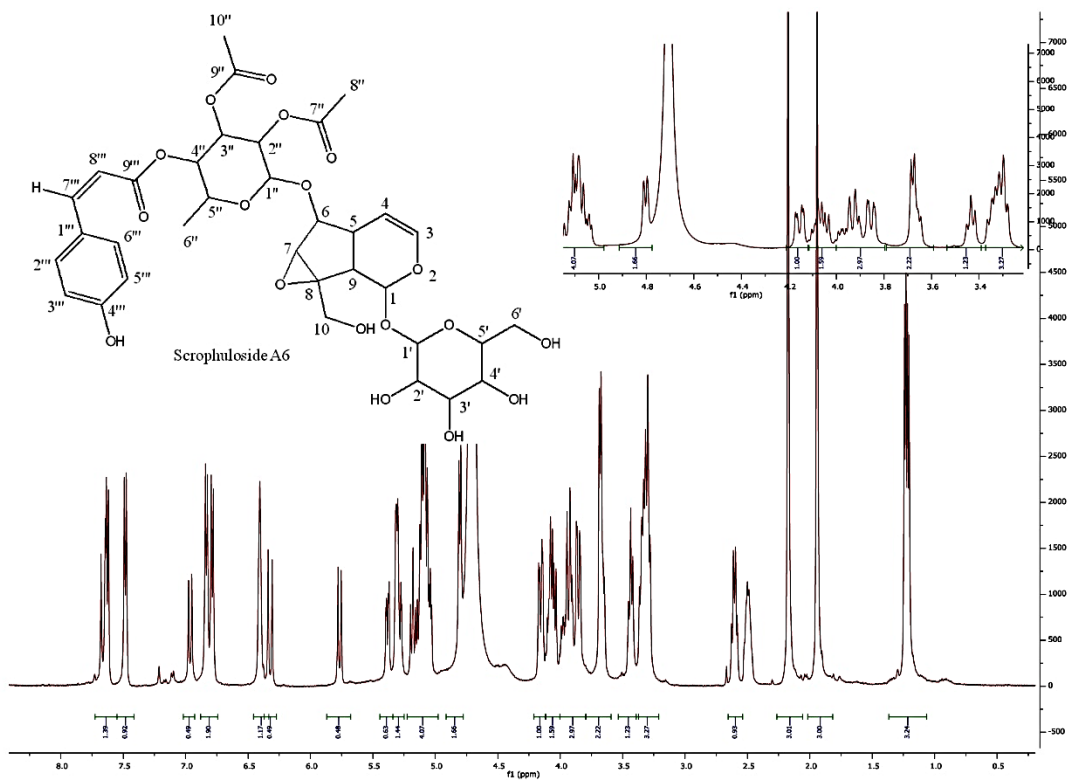
Fig. 15. 1 H-NMR spectrum of Scrophuloides A6, 500 MHz, DMSO-D6
