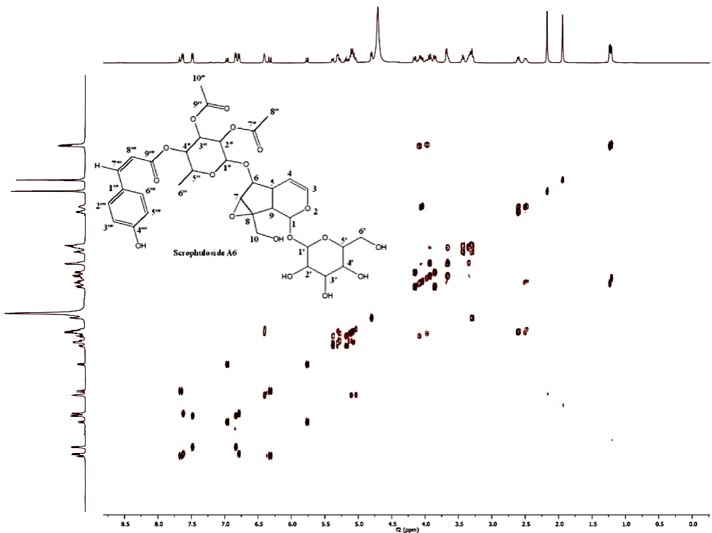
Fig. 16. H-H-COSY spectrum of Scrophuloides A6, 500 MHz, DMSO-D6
