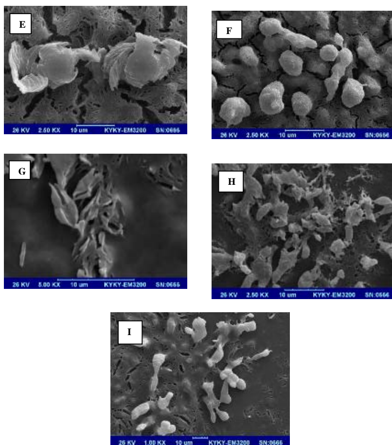
Figure 1- SEM micrograph of electrospayed solution containing different concentration of Menthol and PEG
