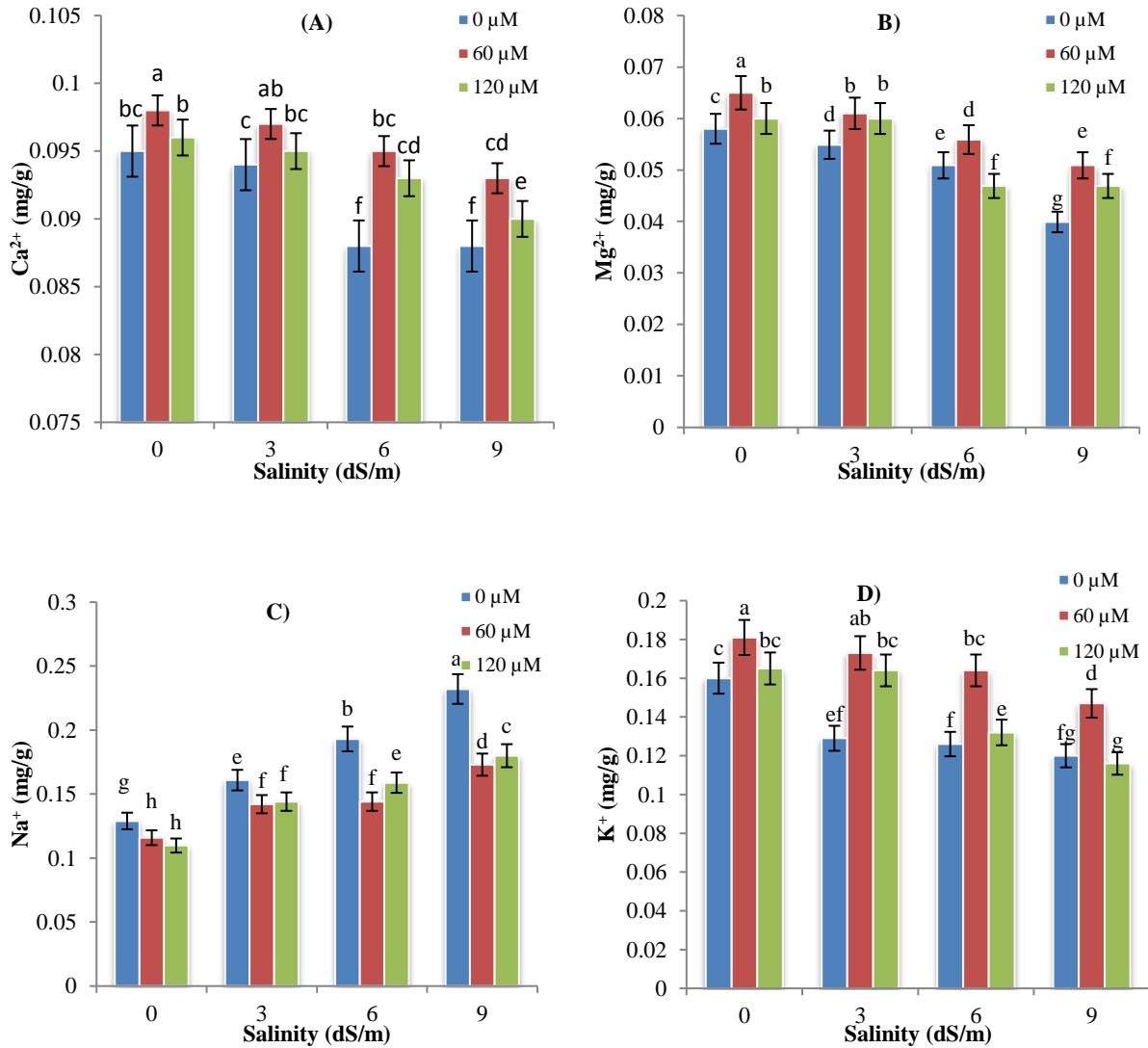
Fig. 2. Effects of salt \times MeJA interaction on mineral elements A: \text{Ca}^{2+} , B: \text{Mg}^{2+} , C: \text{Na}^{+} , D: \text{K}^{+} , E: \text{K}^{+}/\text{Na}^{+} , F: N and G: P in S. khuzistanica . Averages with the same letters are not significantly different and error bars represent standard deviation.
