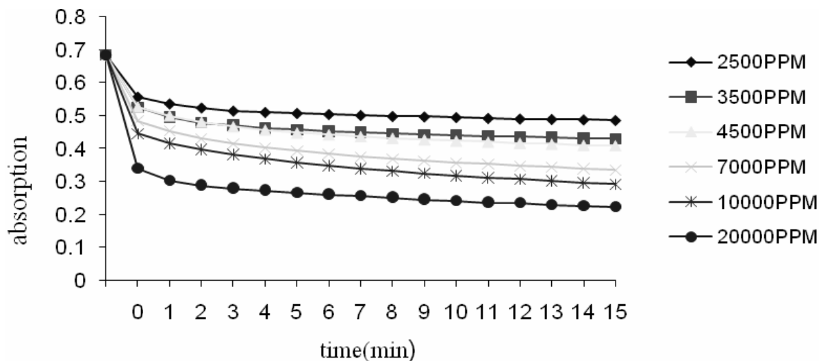
Figure 2- ABTS o+ scavenging activity of BPEO vs. time plots
